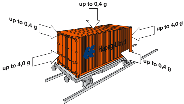
Potential acceleration during rail transport
